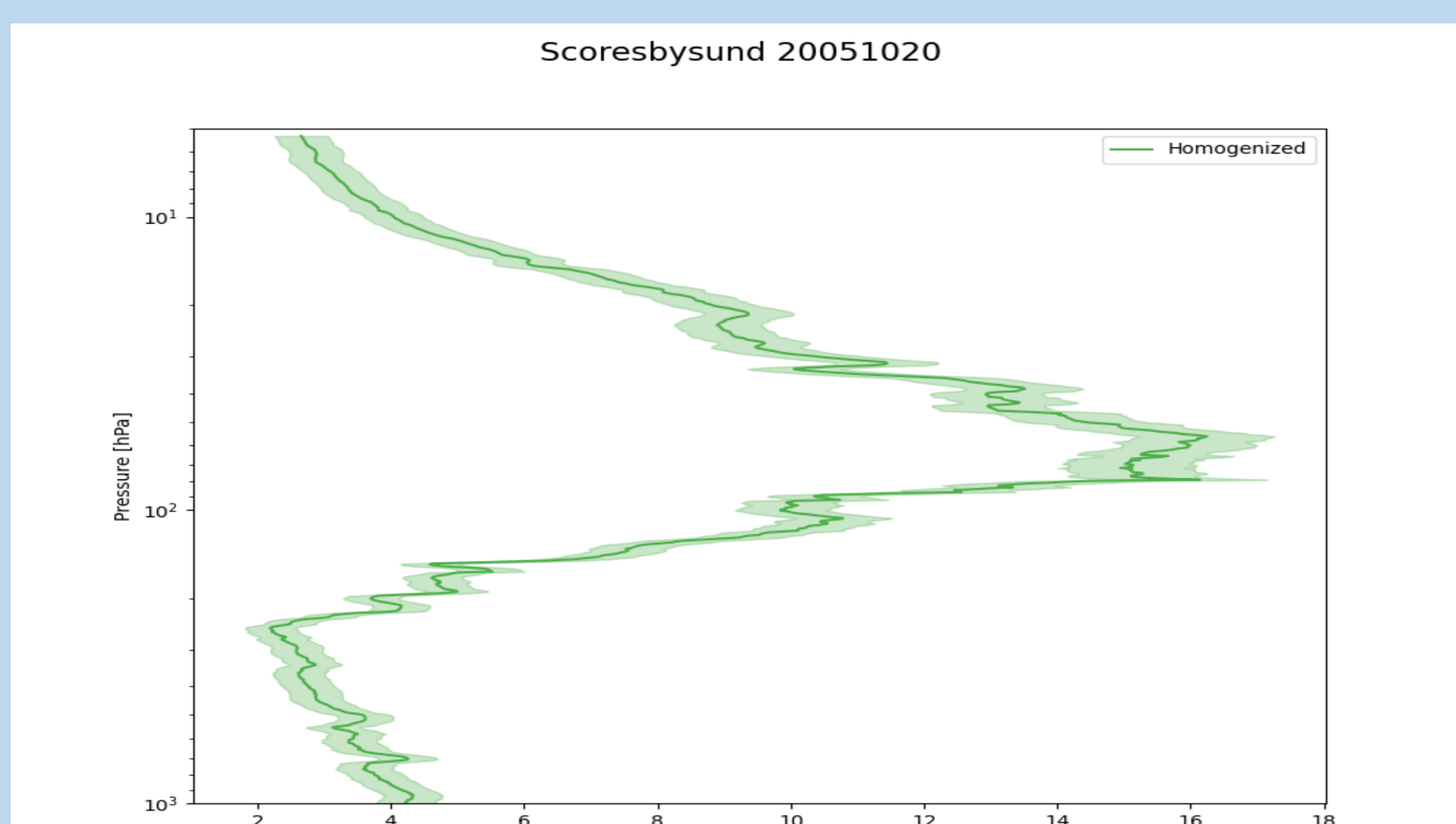
Fig. 2: Ozone sounding at Scoresbysund on 20 October 2005 (green line). The shaded area denotes the estimated uncertainties.
