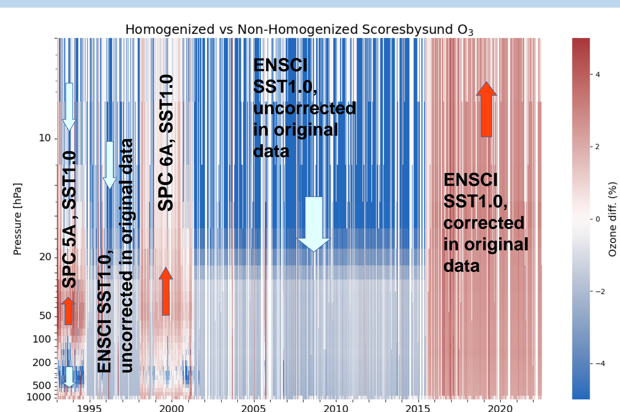
Fig. 1: Relative differences in the vertical ozone concentrations between the homogenized and (minus) non-homogenized ozonesonde time record at Scoresbysund, Greenland. Marked are the used ozonesonde types (SPC 5A, SPC 6A & EN-SCI), and sensing solution type (SST1.0). Note that the recommended combinations are SPC SST1.0 and EN-SCI SST0.5, so that a conversion is needed from the used EN-SCI SST1.0.
