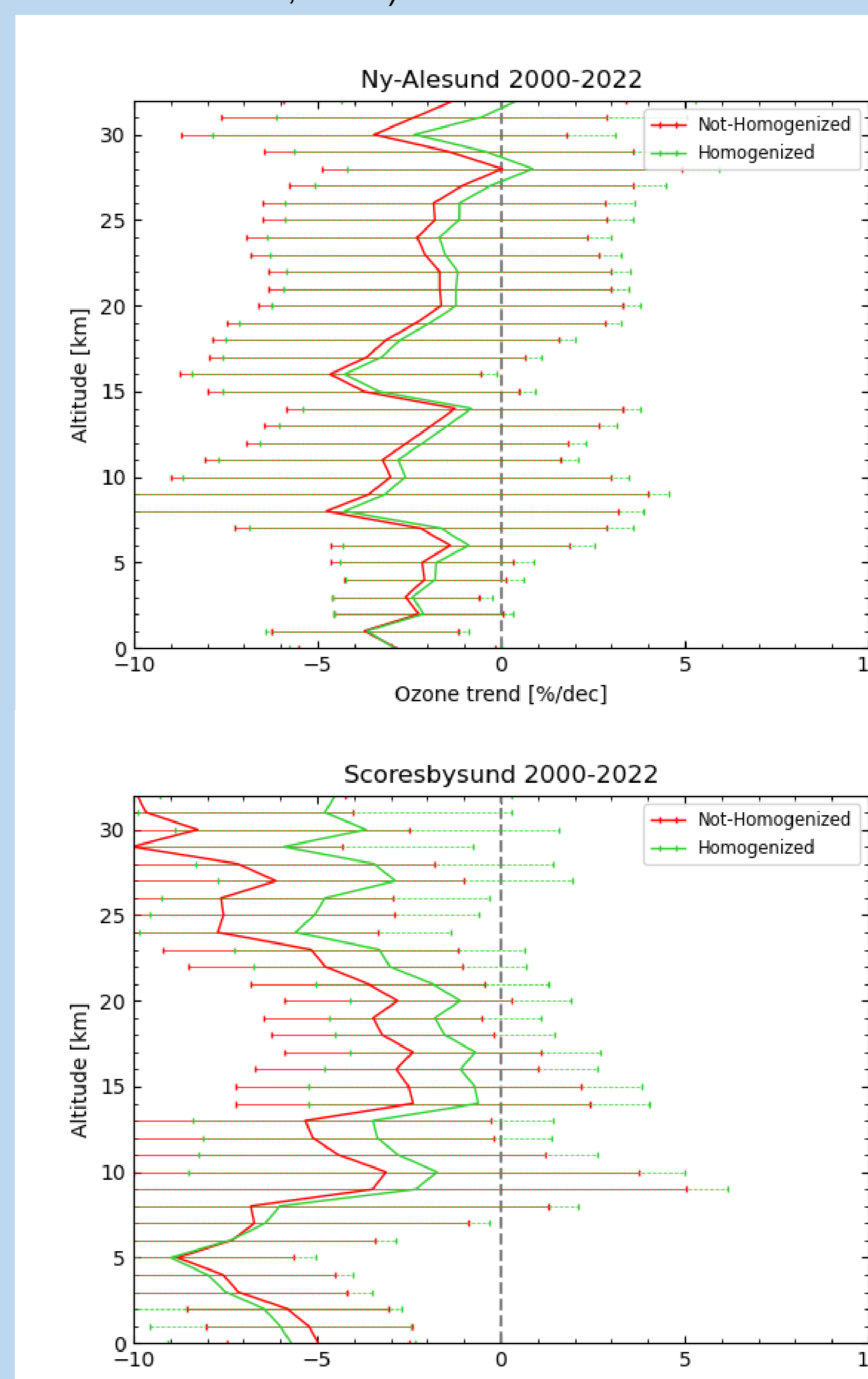
Fig. 5: Post 2000 vertical ozone relative trends [%/dec] estimated with the LOTUS MLR trend model for the Homogenized and Non-Homogenized time series for the Arctic stations Ny Alesund (upper panel) and Scoresbysund (lower panel).
